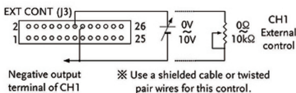
External Voltage Control of the output
